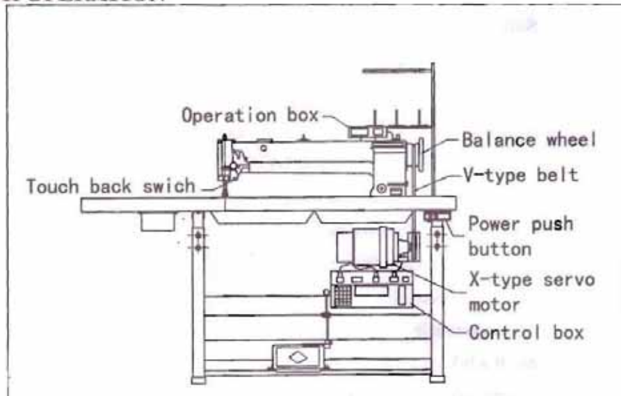
Overall view of assembled sewing machine
